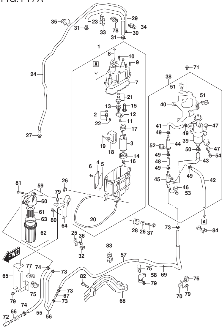
DF350A_000_018_147A FUEL PUMP/FUEL VAPOR SEPARATOR
