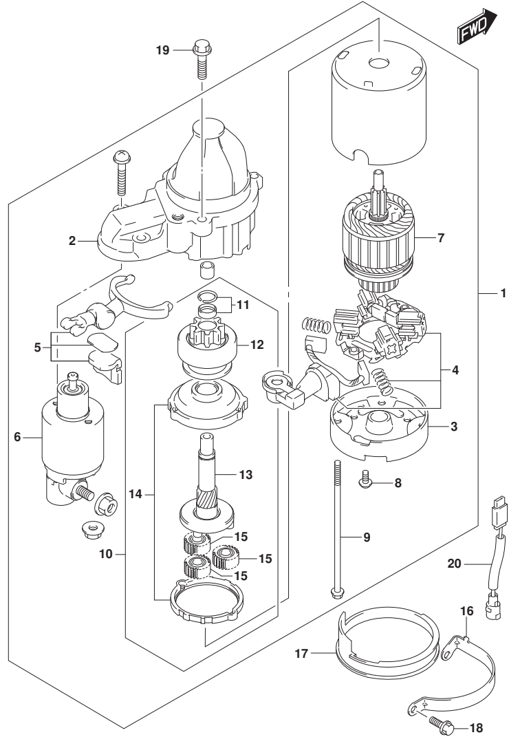
DF300A_000_023_301A STARTING MOTOR
