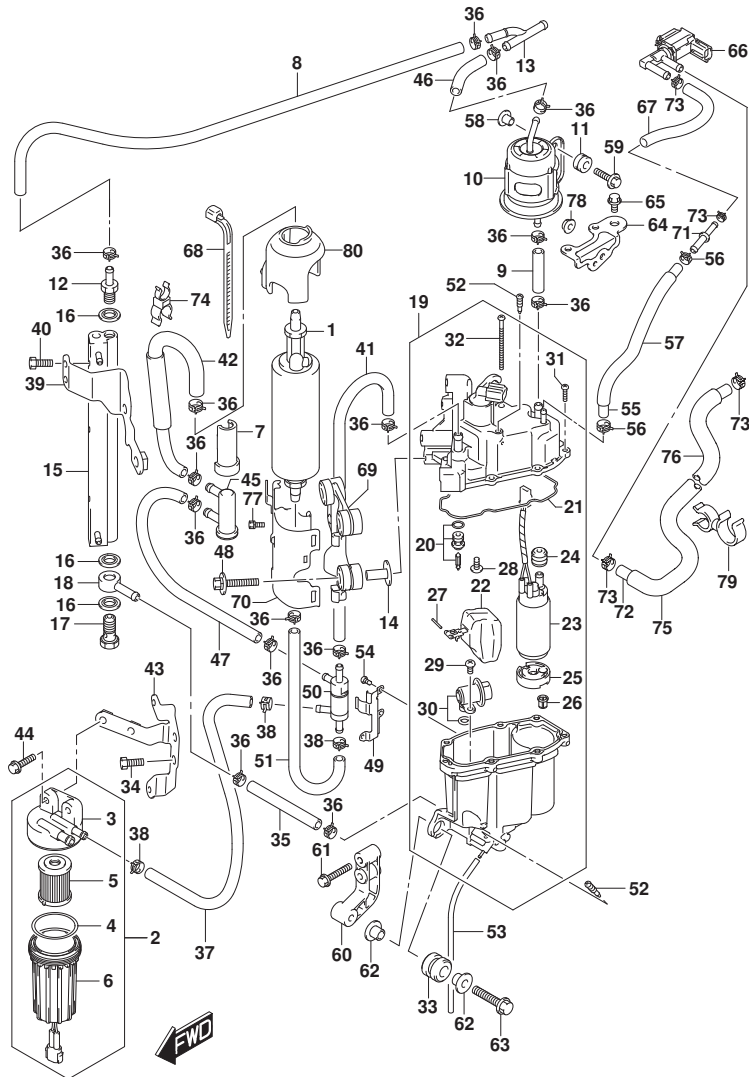
DF300A_000_023_147B FUELPUMP/FUEL VAPOR SEPARATOR
