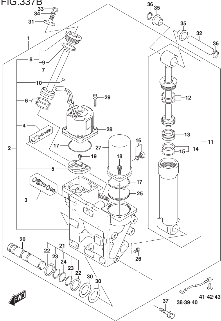
DF250_000_023_337B TRIM CYLINDER
