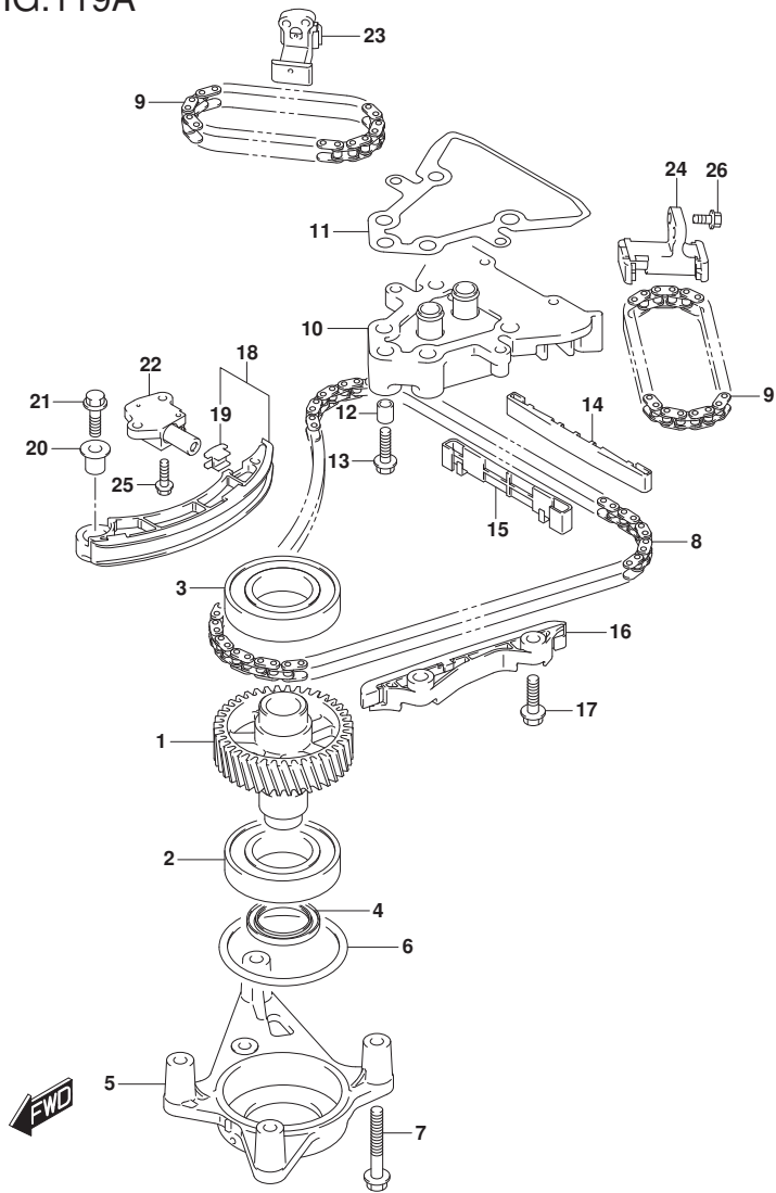
DF250_000_023_119A TIMING CHAIN
