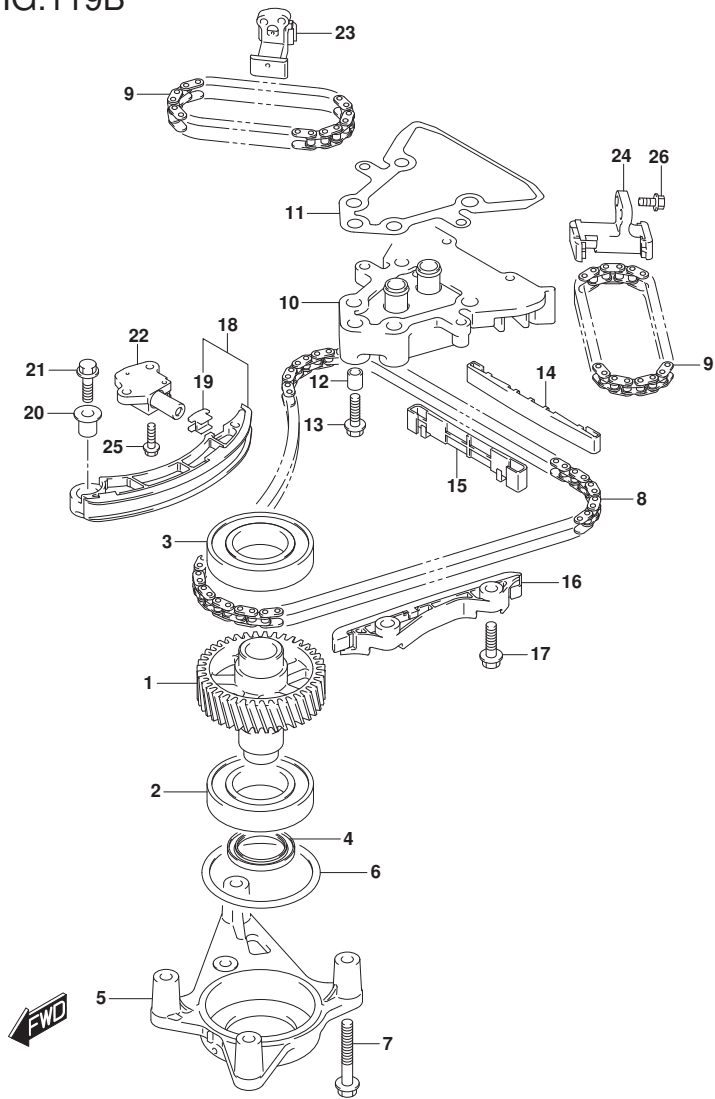
DF250_000_023_119B TIMING CHAIN
