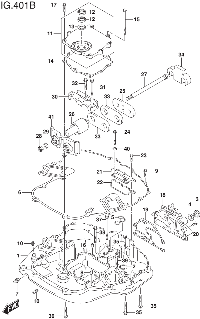
DF250_000_023_401B ENGINE HOLDER
