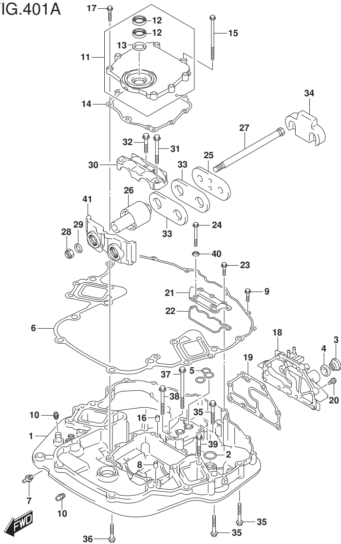
DF250_000_023_401A ENGINE HOLDER
