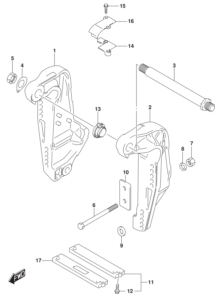
DF250_000_023_335A CLAMP BRACKET
