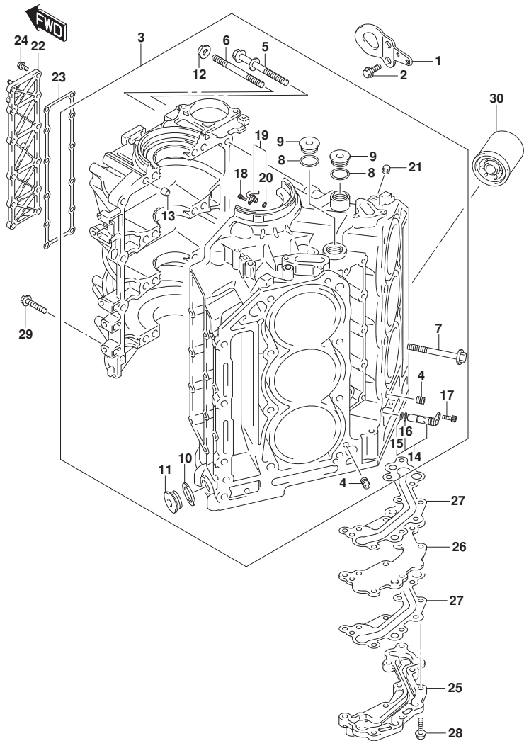
DF300A_000_017_113A CYLINDER BLOCK
