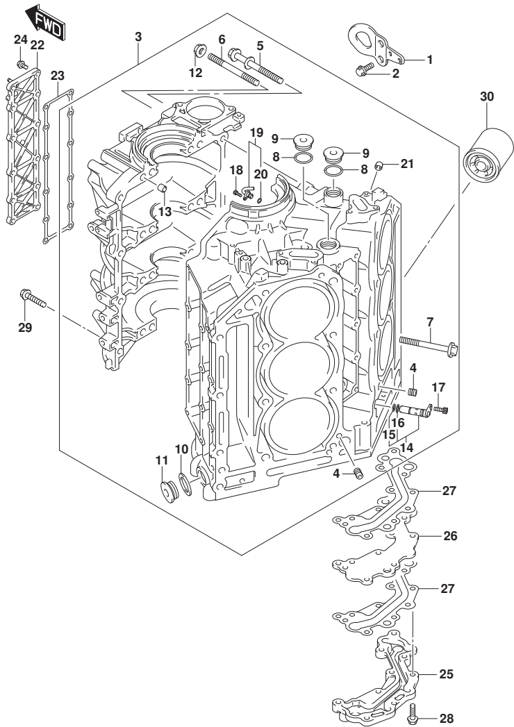
DF300A_000_015_113A CYLINDER BLOCK
