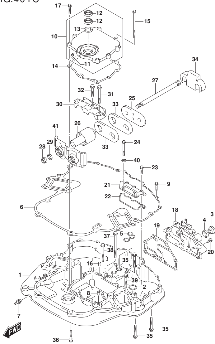
DF250_000_019_401C ENGINE HOLDER
