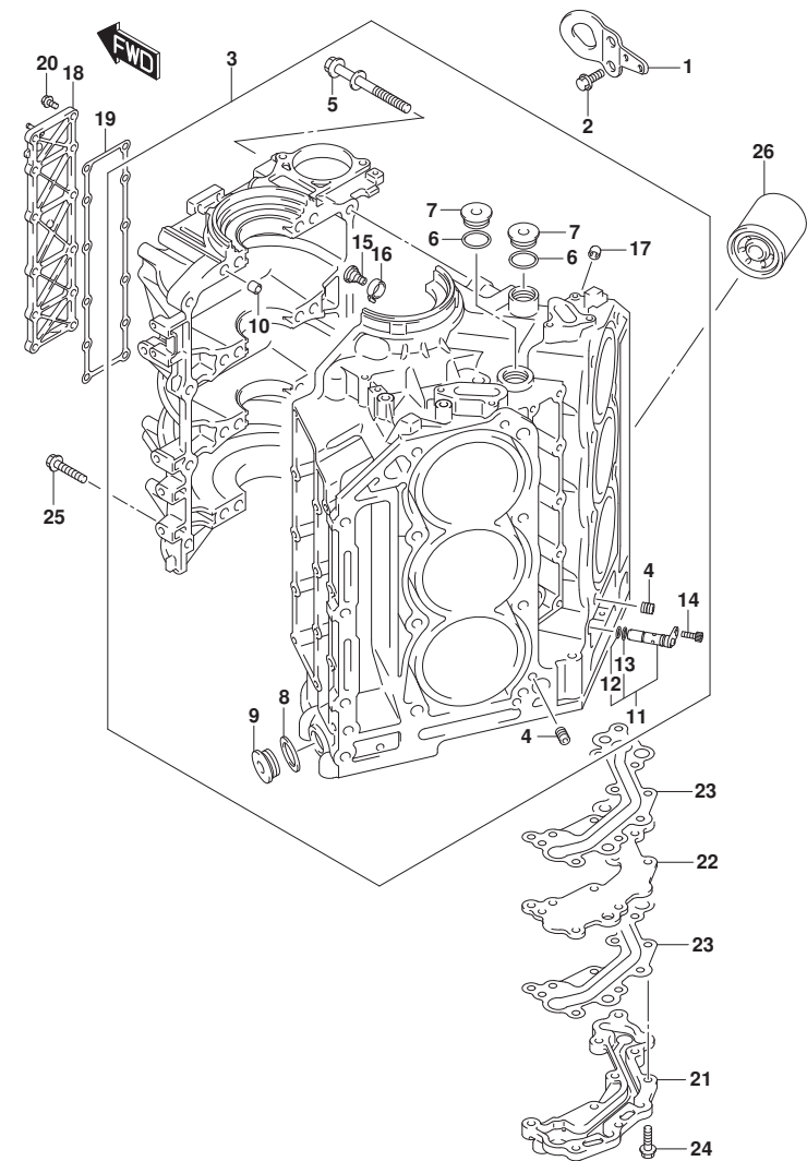
DF250_000_017_113A CYLINDER BLOCK
