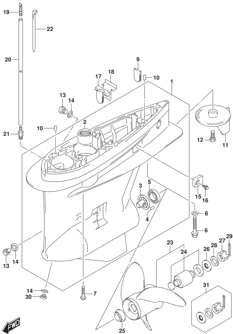
DF200AP_000_016_407A GEAR CASE
